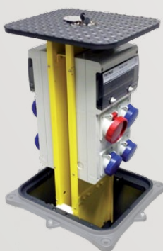
B4030 60 400 x 300 x 600 mm
